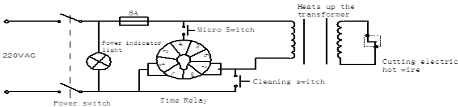
L-type cutting machine circuit diagram
